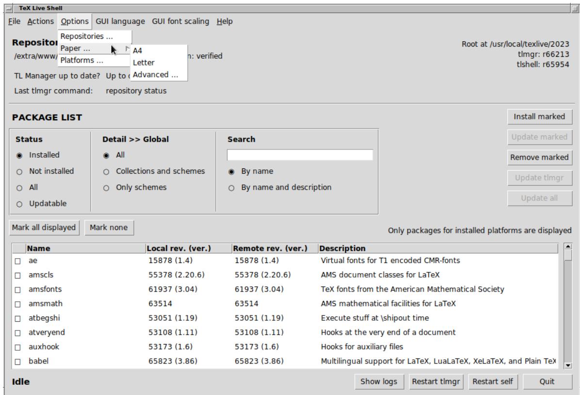
FIGURE 9 – GUI tshell, montrant le menu Actions (GNU/Linux)
